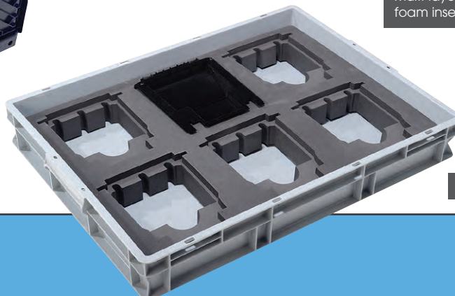
Water jet & fabricated foam insert
